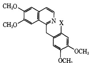
3a, X = Br b, X = CH 2 COCH 3
